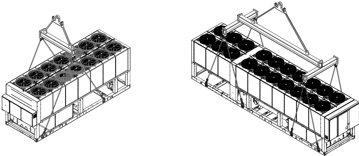
Figure 3 - Lifting the unit
