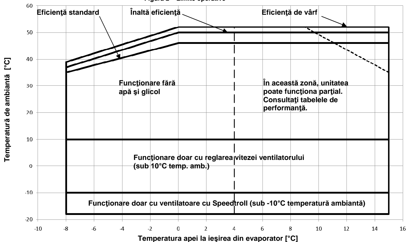
Figura 2 – Limite operative
